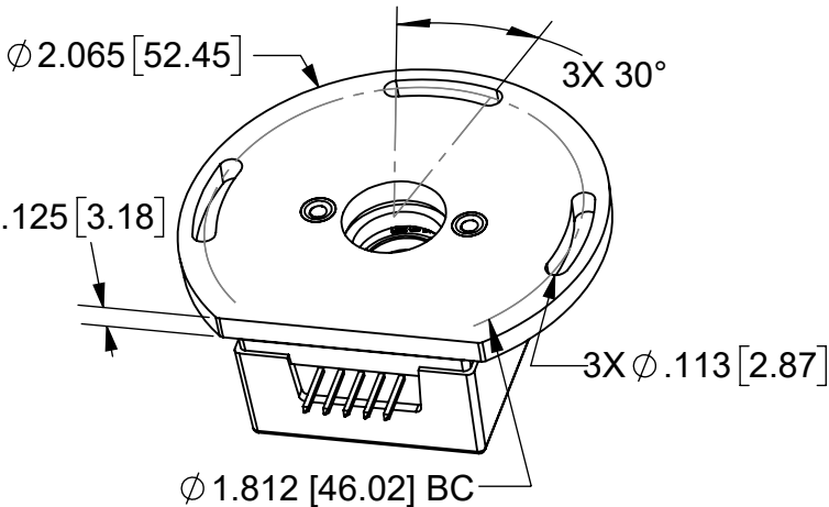
R-OPTION BASE (ROTATIONAL MOUNTING)
