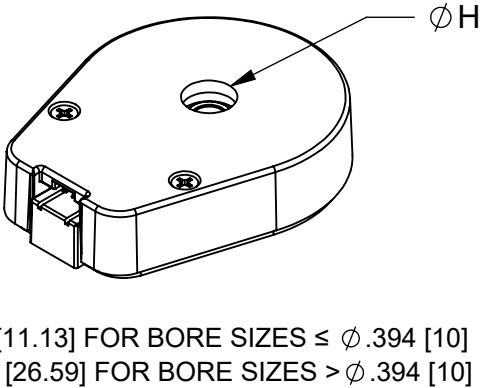
H-OPTION COVER (COVER HOLE FOR SHAFT LENGTHS OVER .750 [19.05])
