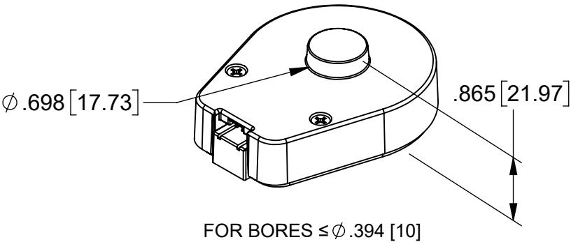
E-OPTION COVER (EXTENSION FOR SHAFT LENGTHS UP TO .750 [19.05])
