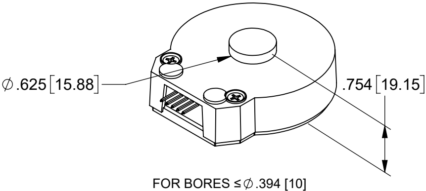
E-OPTION COVER (EXTENSION FOR SHAFT LENGTHS UP TO .670 [17.02])
