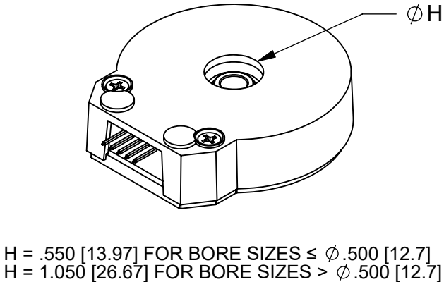
H-OPTION COVER (COVER HOLE FOR SHAFT LENGTHS OVER .670 [17.02])
