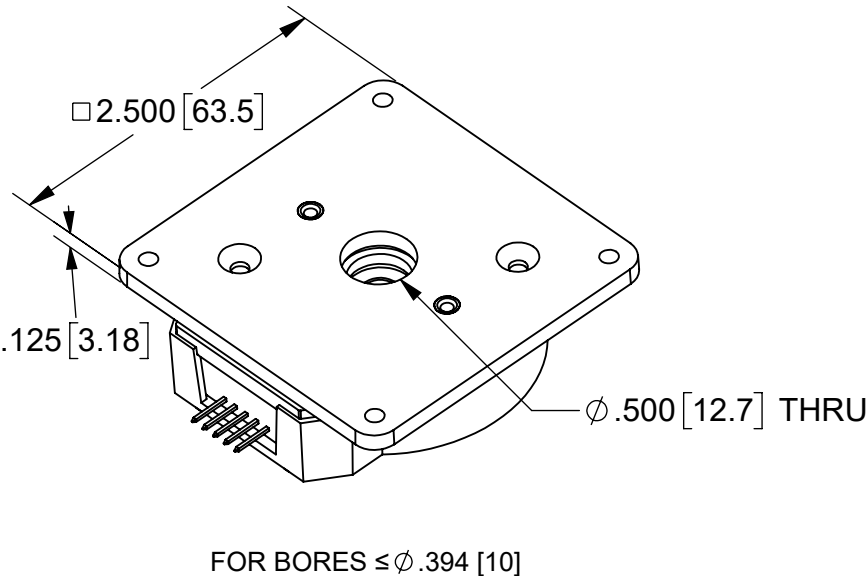
M-OPTION BASE (MOUNTING PLATE) REQUIRES MINIMUM .570 [14.48] SHAFT LENGTH
