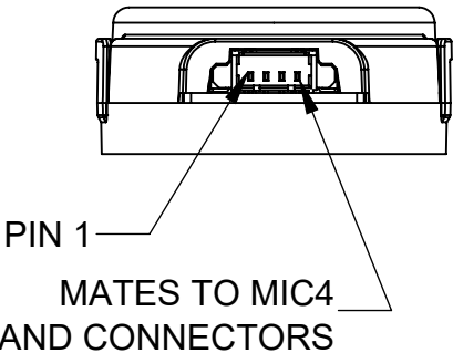
SINGLE-ENDED VERSION (4-PIN)
