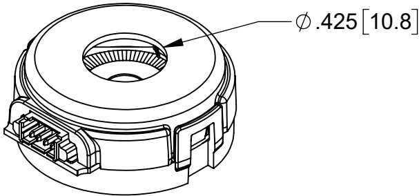
H-OPTION COVER (COVER HOLE FOR SHAFT LENGTHS OVER .400 [10.16])
