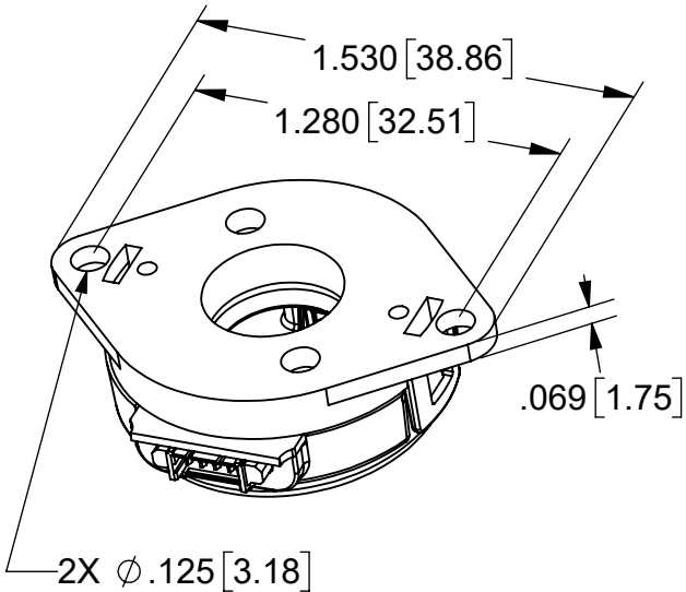
G-OPTION BASE (1.280 MOUNTING)
